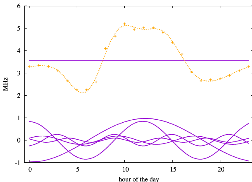
Fig. 3. Fourier decomposition of the daily variation (UT) of foF_2 for January for F_{10.7} = 67.5 sfu. The dashed line is the modeled diurnal variation; the crosses present the measured monthly median values and the solid lines – the harmonics used in the decomposition together with the constant component (the straight line).
